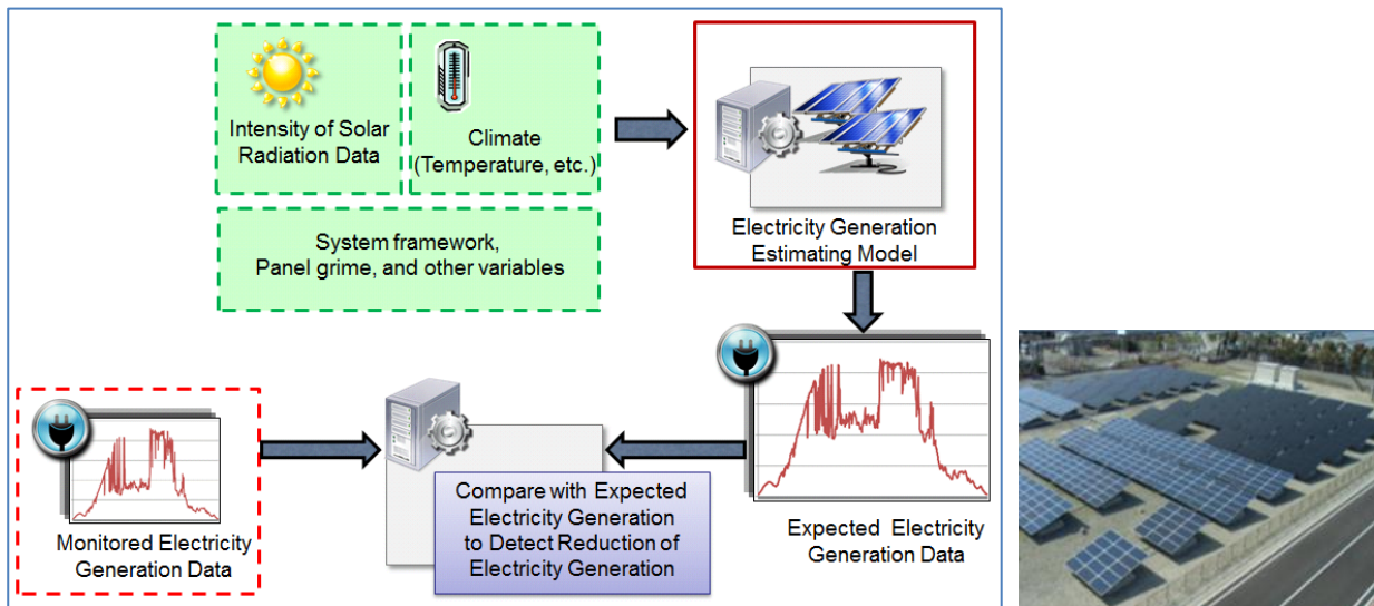
left) Trouble flow right) Solar generation test facility at Mitsui Chemical Mobara Works
